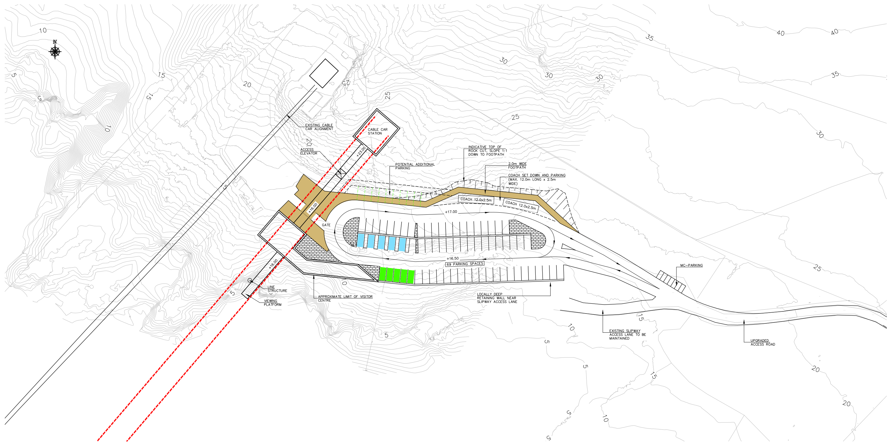
OPTION 3 – MAINLAND SITE LAYOUT PLAN
